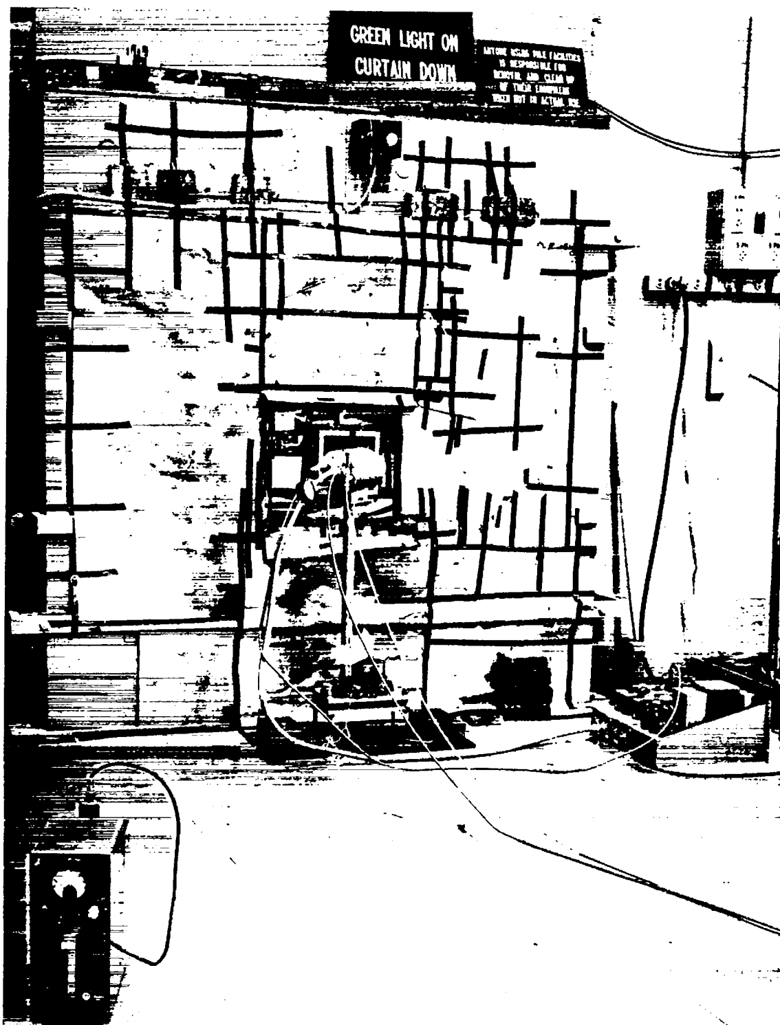
Fig. 3. The south face of the Water Boiler with fission chamber in place.
