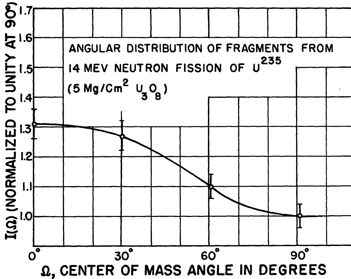
Fig. 10. Angular distribution of fragments from the 14-Mev fission of U^{235} .
