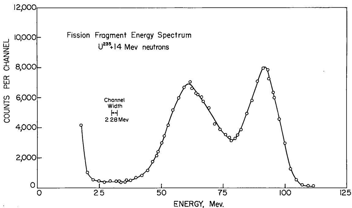
Fig. 6. Fission fragment energy spectra for thermal and 14-Mev neutrons.
