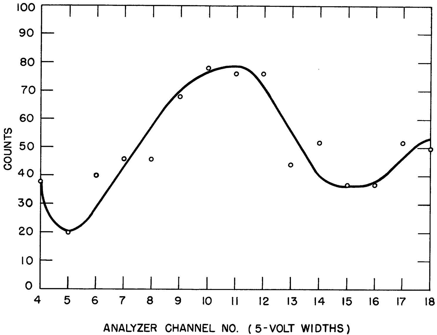
Fig. 9. A pulse height spectrum taken with 14-Mev neutrons.
